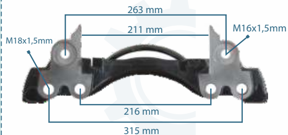
133225 CALIPER CARRIER 19.5" LEFT
