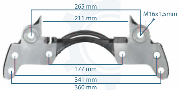
133219 CALIPER CARRIER 19.5" LEFT
