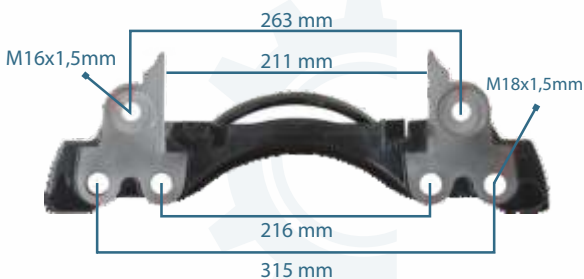
133226 CALIPER CARRIER 19.5" RIGHT
