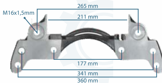
133220 CALIPER CARRIER 17.5" RIGHT
