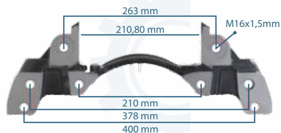
133178 CALIPER CARRIER PAN22 LEFT
